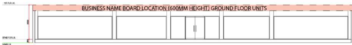
Figure 2: Commercial frontage Elevation with business name board location and dimensions.
